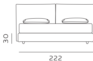
222 materasso largh. cm. 200 mattress width cm. 200
