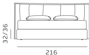
216 materasso largh. cm. 180 mattress width cm. 180
